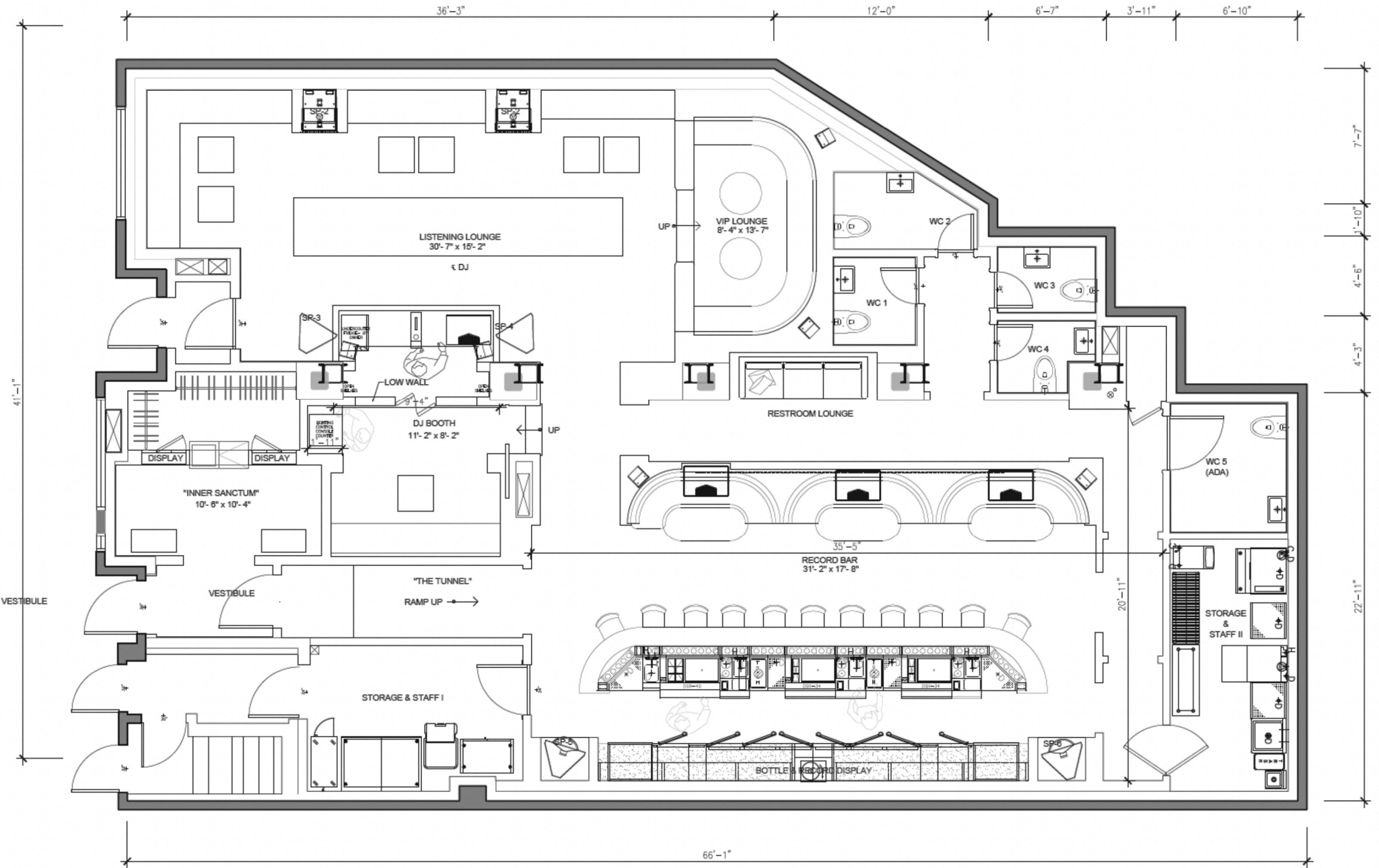
1 FLOOR PLAN SCALE: 3/8"=1'-0"
